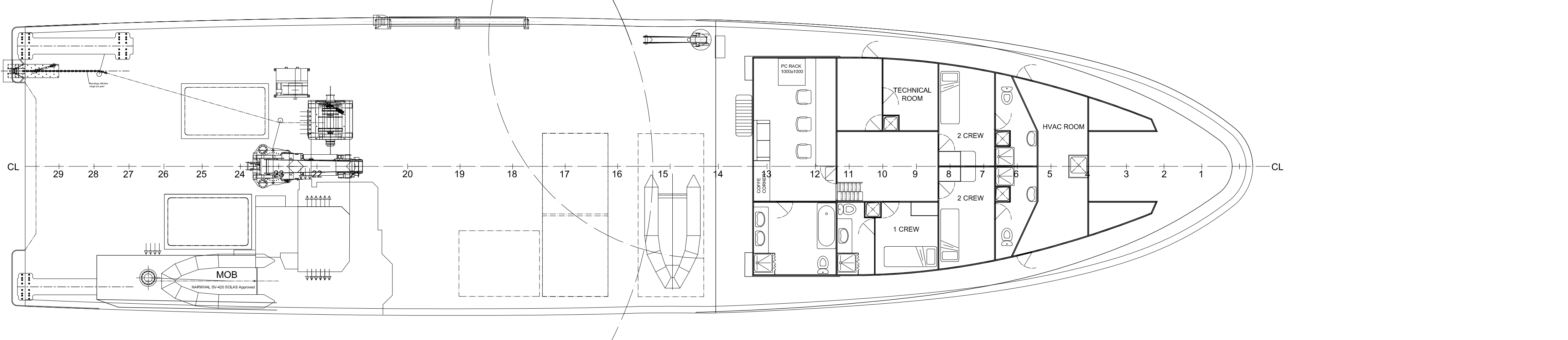
DECK 2 - MAIN DECK
